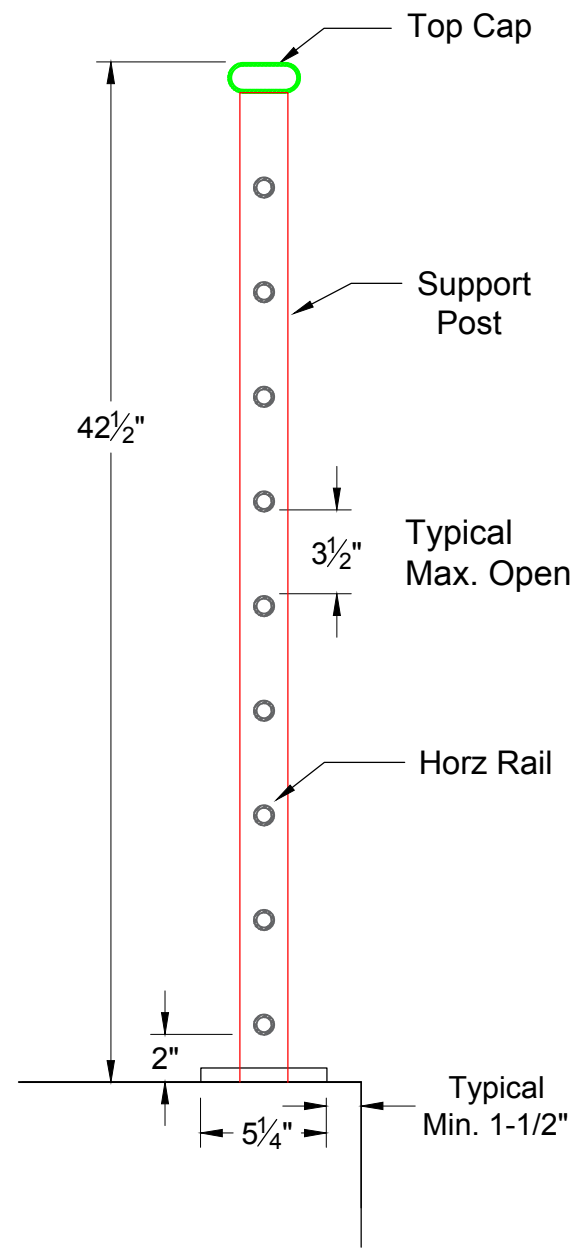
ENLARGED SECTION 1/2" = 1' - 0"
