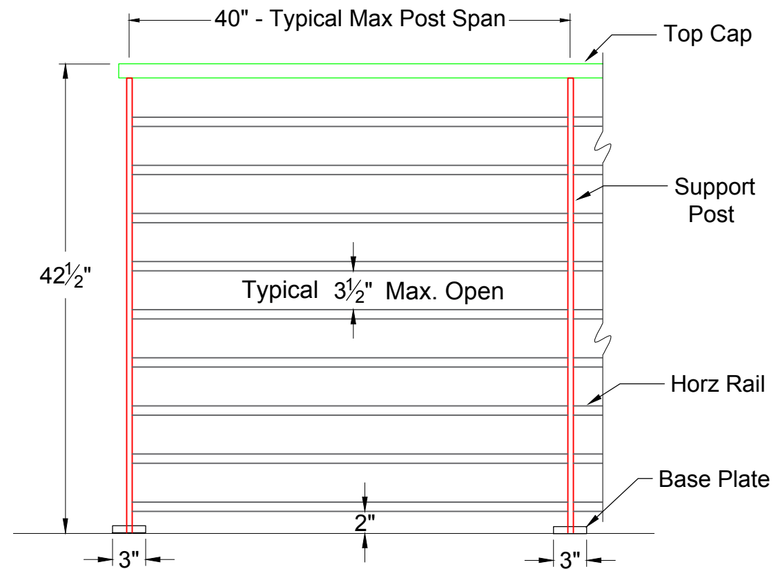
ELEVATION 1" = 1' - 0"
