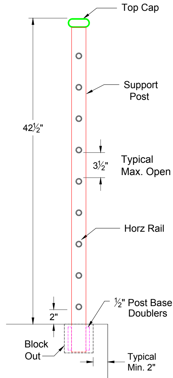
ENLARGED SECTION 1 1/2" = 1' - 0"
