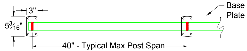
PLAN VIEW 1" = 1' - 0"
