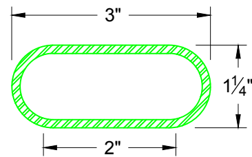
TOP CAP ( SHOWN ) 3" x 1-1/4" OVAL TUBE
