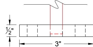
BASE PLATE ELEV.
