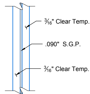
LAMINATED GLASS DETAIL
