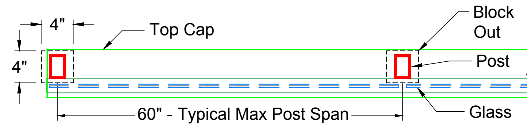
PLAN VIEW 1" = 1' - 0"
