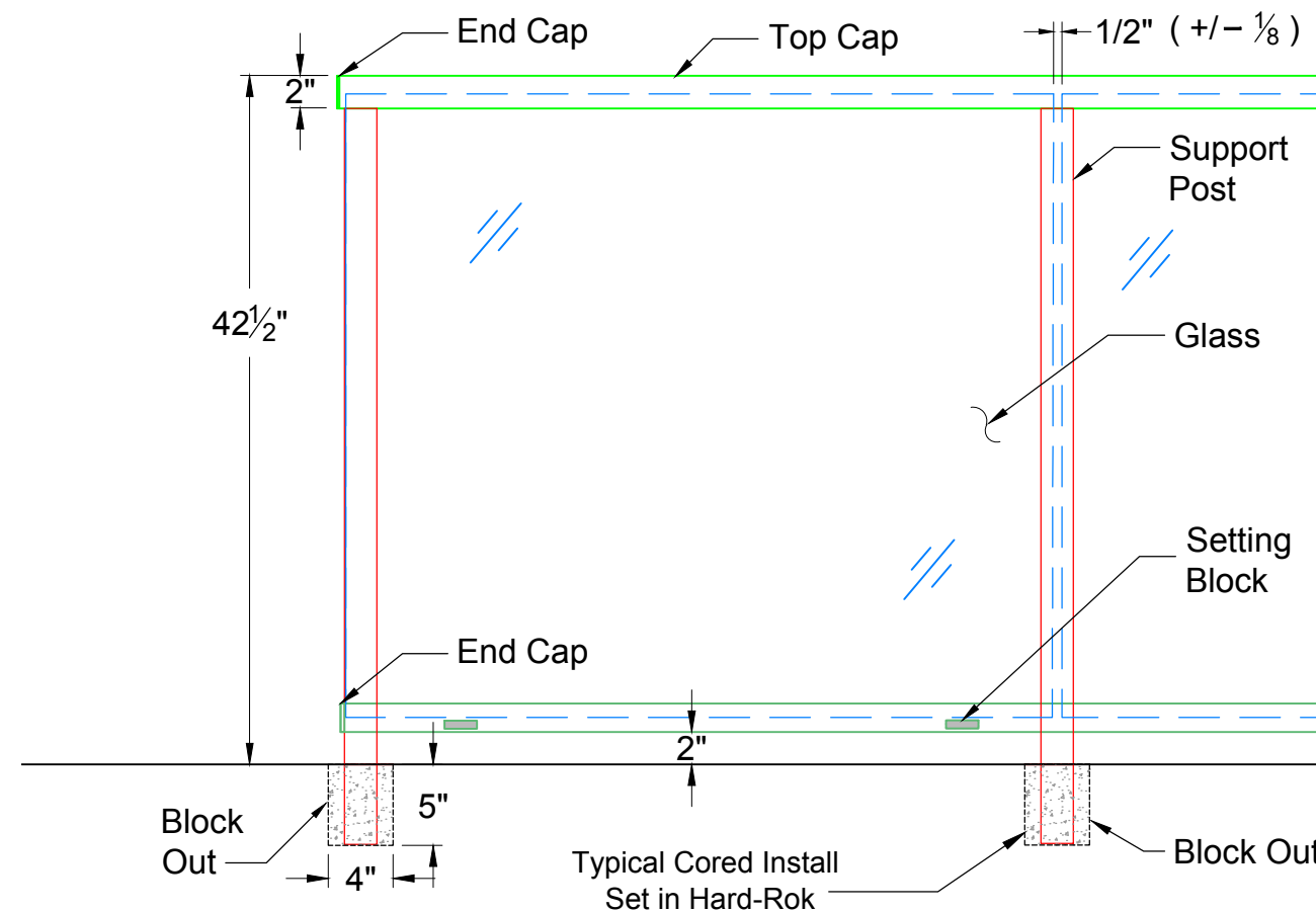
ELEVATION 1" = 1' - 0"
