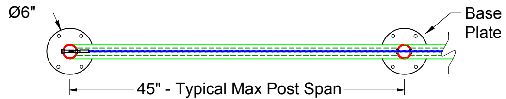
PLAN VIEW 1" = 1' - 0"
