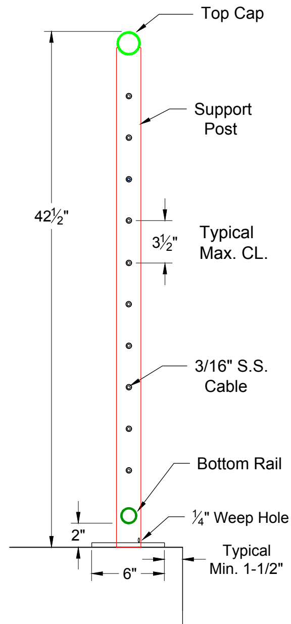
ENLARGED SECTION 1/2" = 1' - 0"
