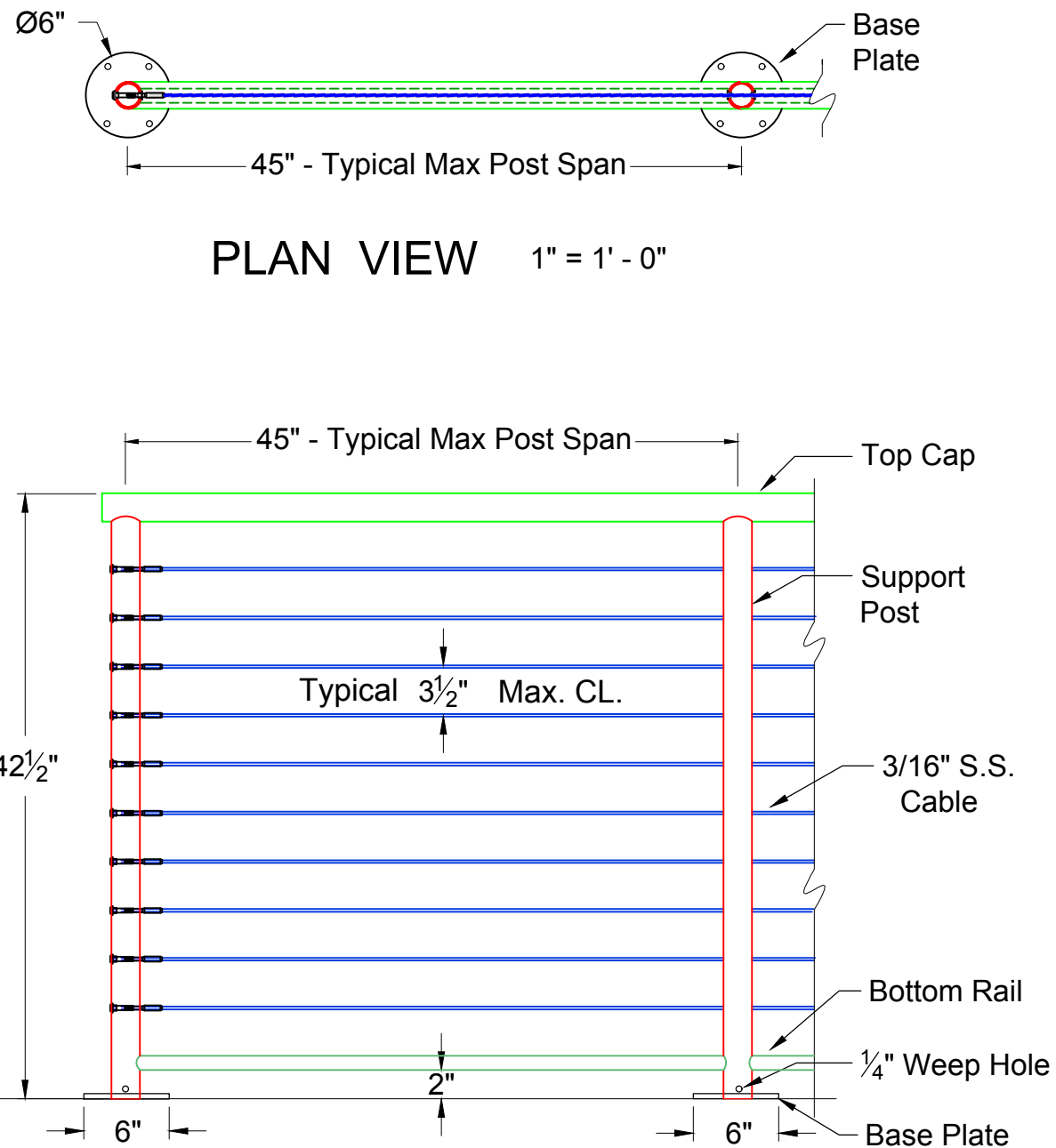
ELEVATION 1" = 1' - 0"
